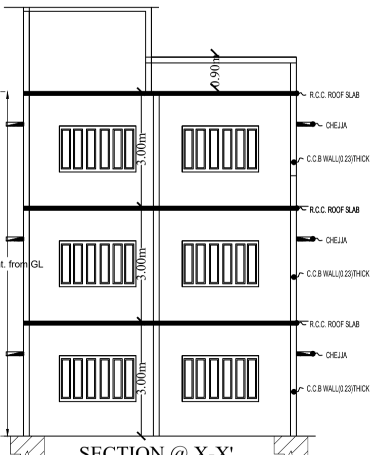
SECTION @ X-X'
